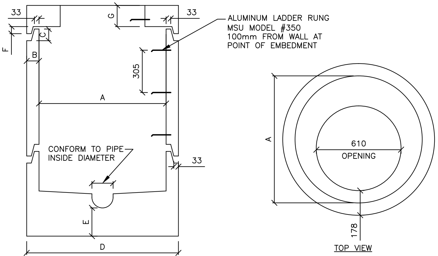
MANHOLE PRE-BENCHED BASE SCALE: NTS
